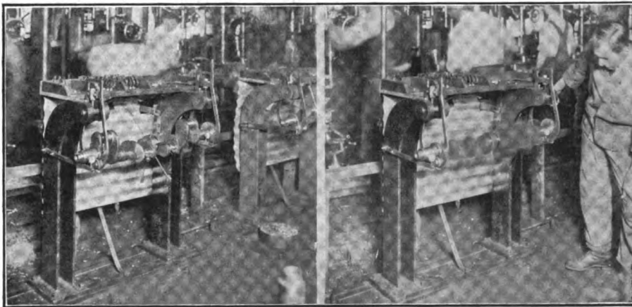
Continental dynamic balancing machine. At left, crankshaft ready for testing; at right, shaft revolving under pressure of pneumatic blast
